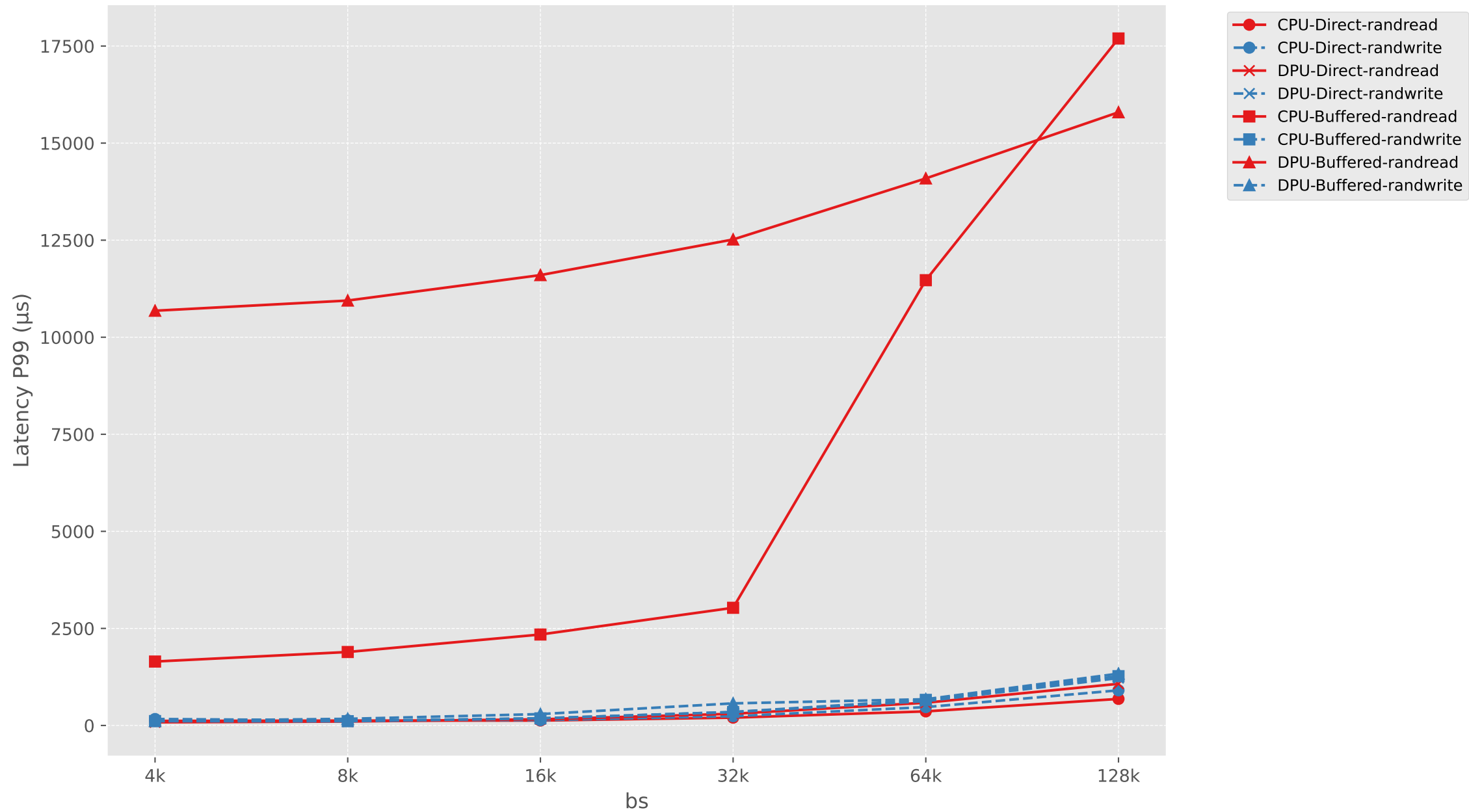
Latency P99 vs bs (CPU vs DPU, Direct vs Buffered)
